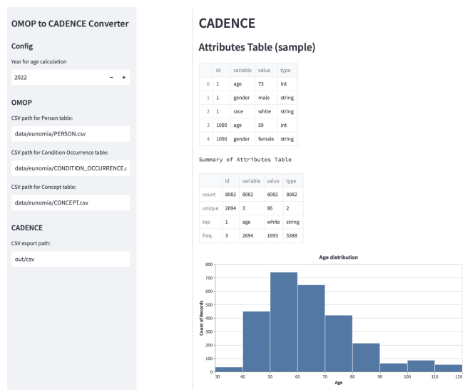
Fig. 2. A partial screenshot of the web-based application with a data quality report on the right panel. Users can edit configuration settings on the left panel of the application.
